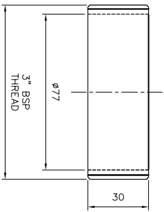
(SCALE 1:4) DETAIL-A BUSH FOR COUPLER
